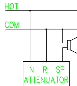
2-WIRE CONNECTION
