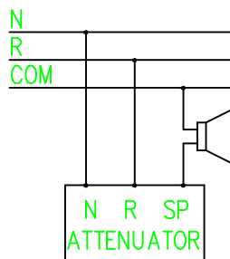
3-WIRE CONNECTION
