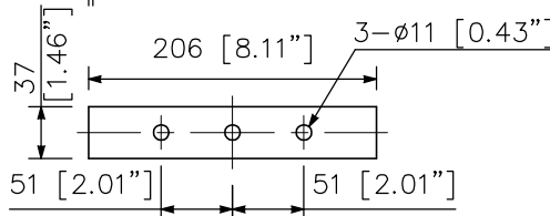
Bracket dimensional diagram
