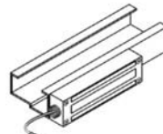
INSTALLATION OF MAGLOCK BODY ON DOOR FRAME
